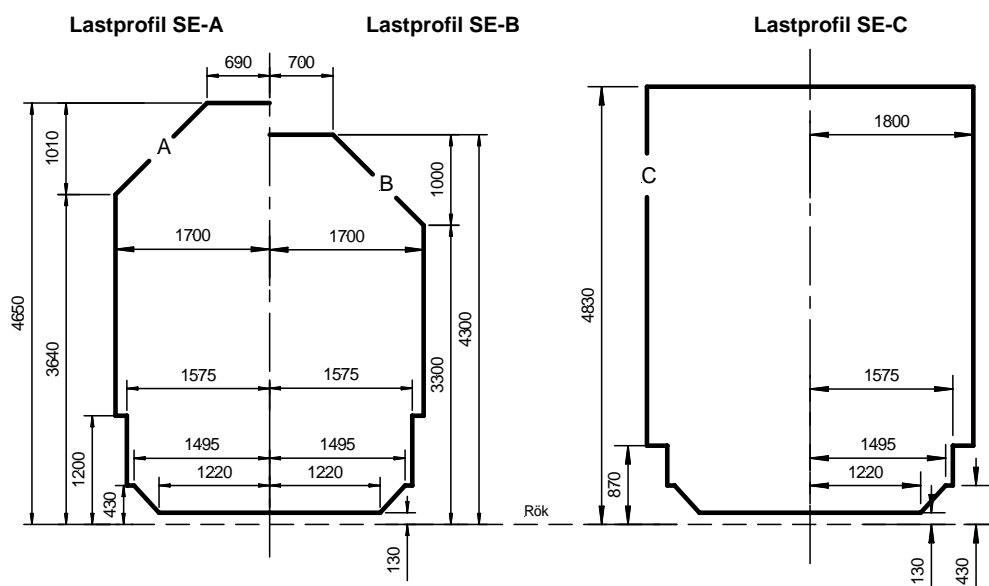
Figur 3.1 Lastprofiler
