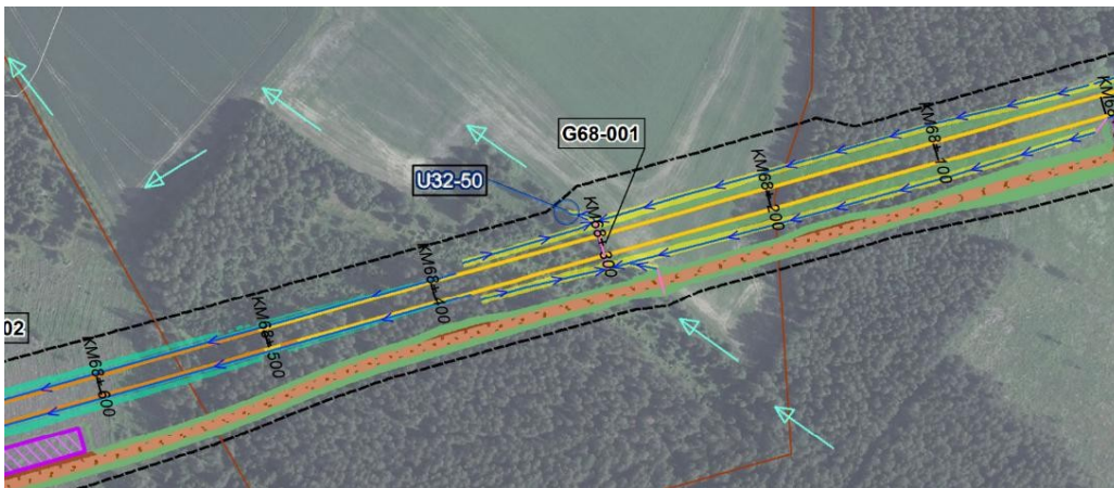
Figure C1.12. Discharge point to the Ängsäter–Brottninge temporary land drainage scheme.
