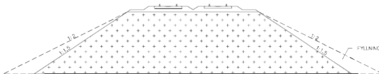
Figure (G).2 Transition structure for ballasted track system, section 1
