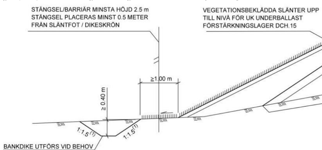
Figure (FB73).1. Schematic diagram showing how a bank ditch can be positioned for a low embankment
