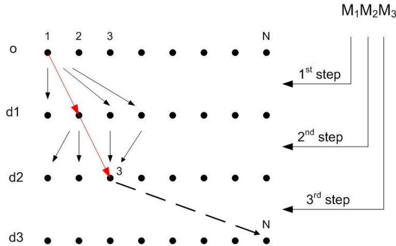
Figure 3: Search algorithm, the optimal two leg chain M_1M_2 from origin 1 to destination 3 is indicated in red
