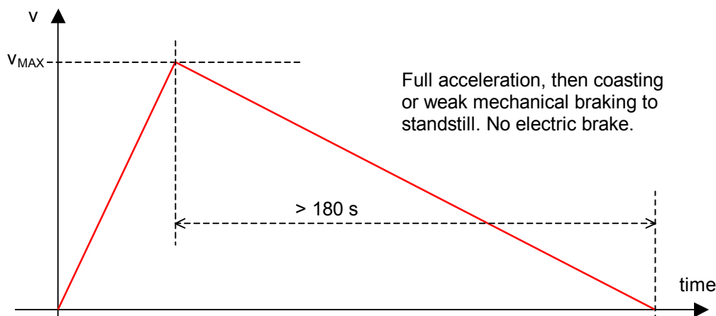
Figure 16. ARO (Acceleration-RollOut) operation sequence.
