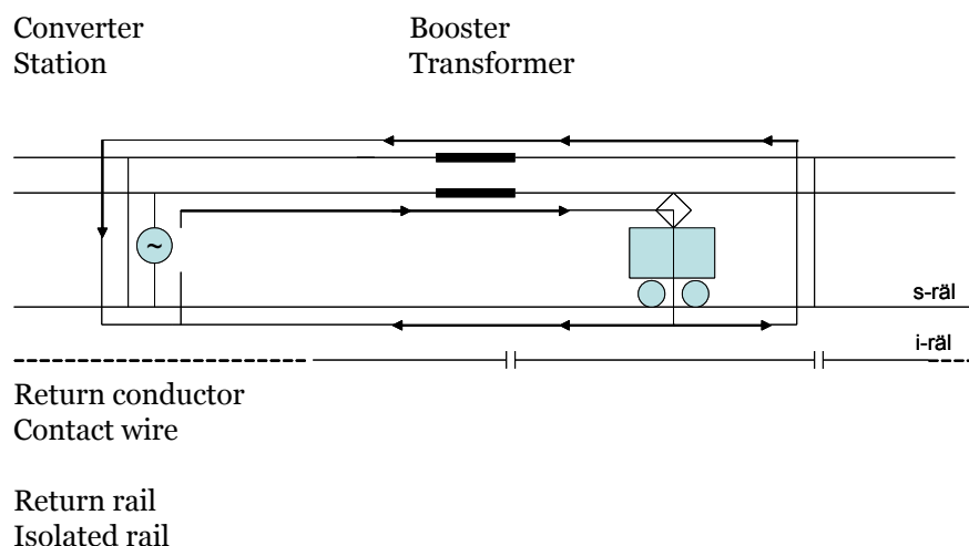
Figure 4. Train position at the inrush current test. For booster transformer data, please refer to Appendix 1, section A1.2.3, A1.2.4 and A1.5.6.
