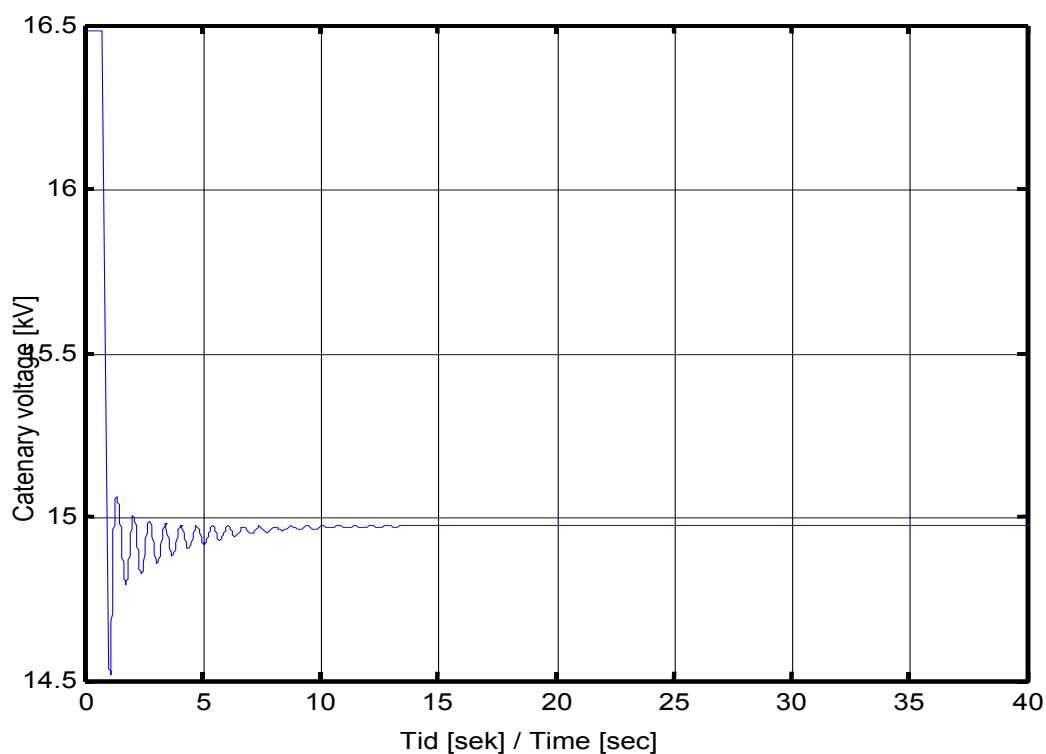
Figure A5-2 U 60km for active power step in the train of 0 – 2.0 MW
