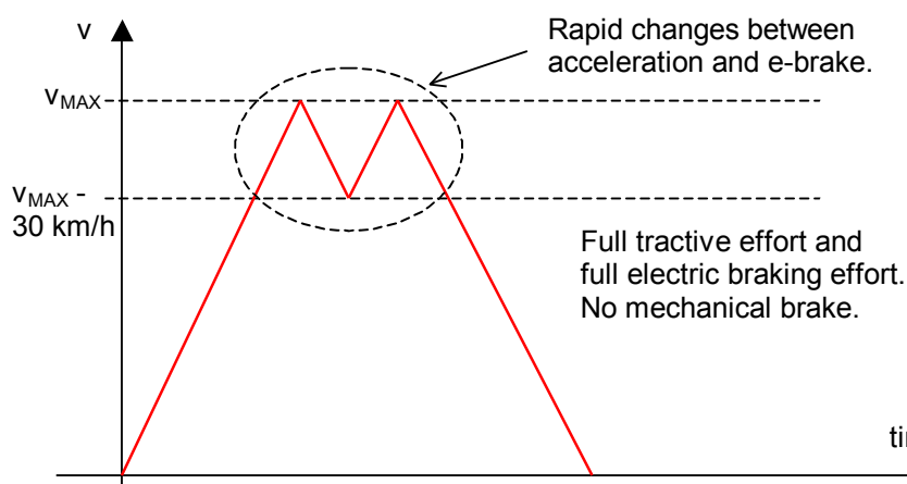
Figure 15. ABAB (Acceleration-Brake-Acceleration-Brake) operation sequence.
