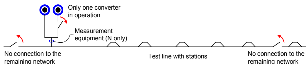
Figure 13. Supply conditions for T1 tests, P-requirements.
