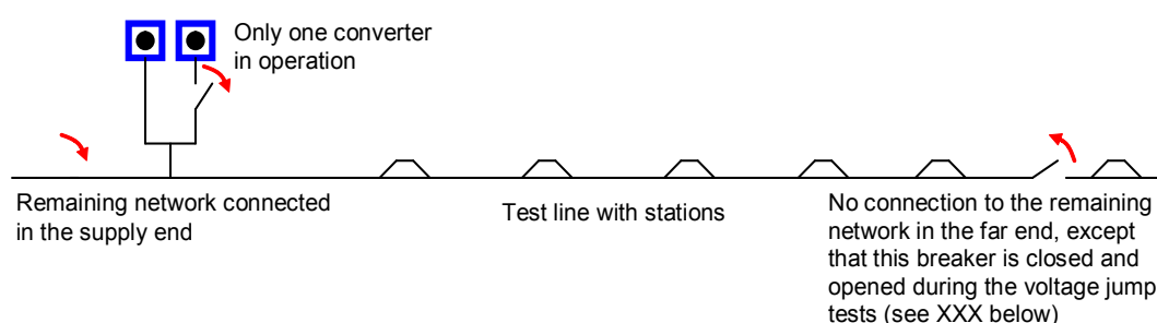
Figure 14. Supply conditions for T2 tests, P-requirements.
