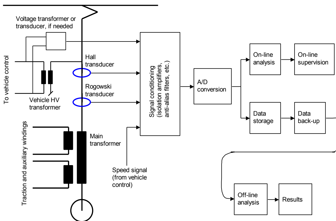
Figure 18. Transducer position and recommended measuring equipment.
