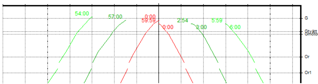
Figure 1. Detailed view of the graph near Göteborg Central during stage 1. An exception to the rule of arrivals and departures at even five-minute intervals is made to allow for three consecutive arrivals, followed by three consecutive departures.
