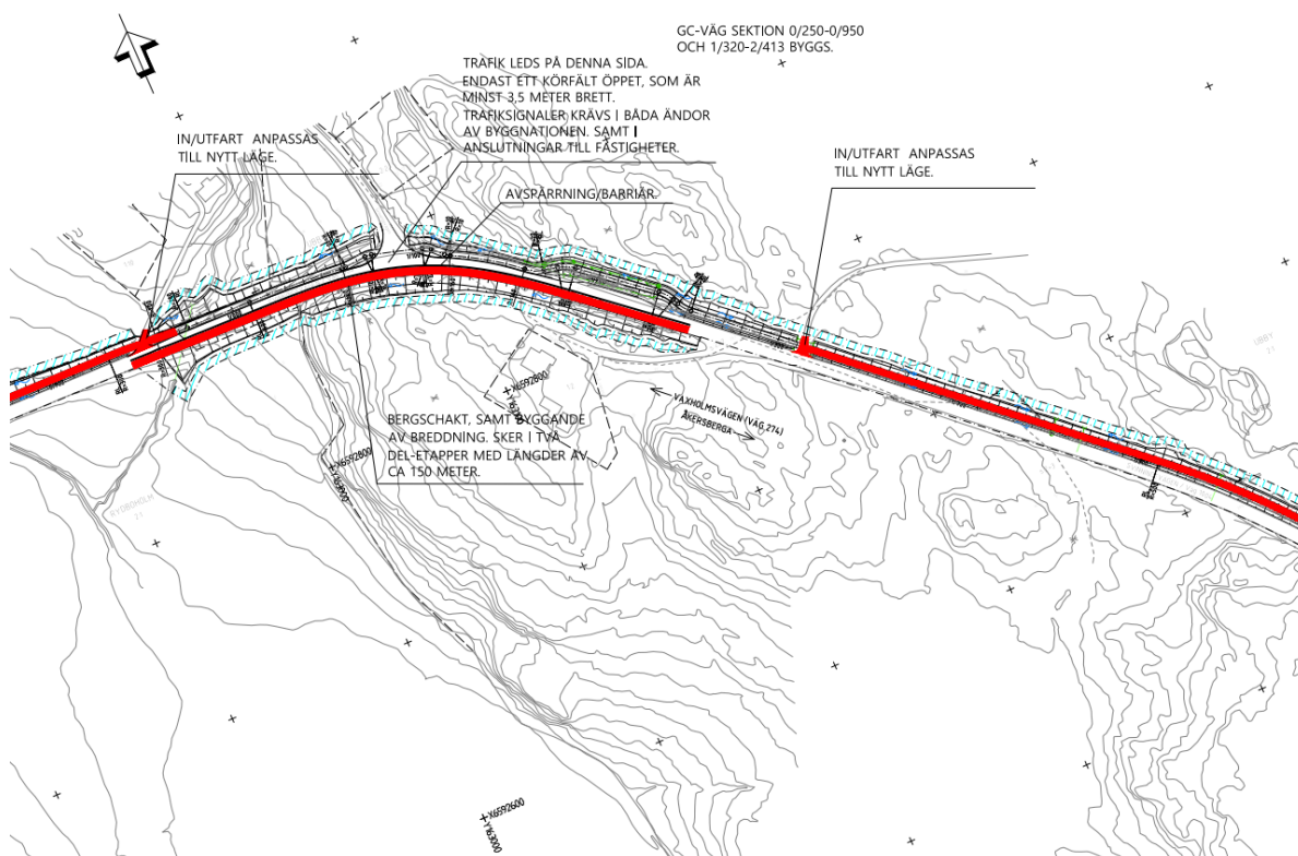
Figur 37. Skedesplan skede 1 TUB B, ritning 100T40B1.
