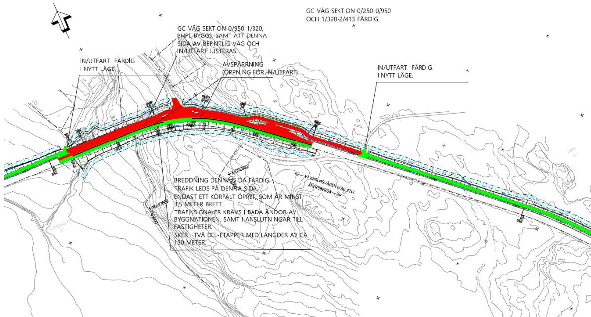
Figur 38. Skedesplan skede 2 TUB B, ritning 100T40B2.
