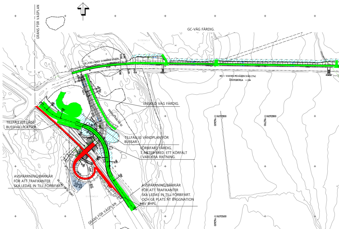
Figur 31. Skedesplan skede 4 TUB A, ritning 100T40A4.
