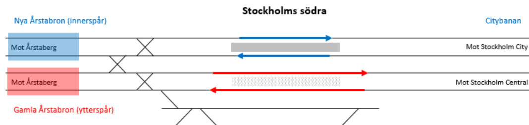
Figure 1: Schematic track plan Stockholm södra. South of Årstadavägen the two double tracks change to one four-track.
