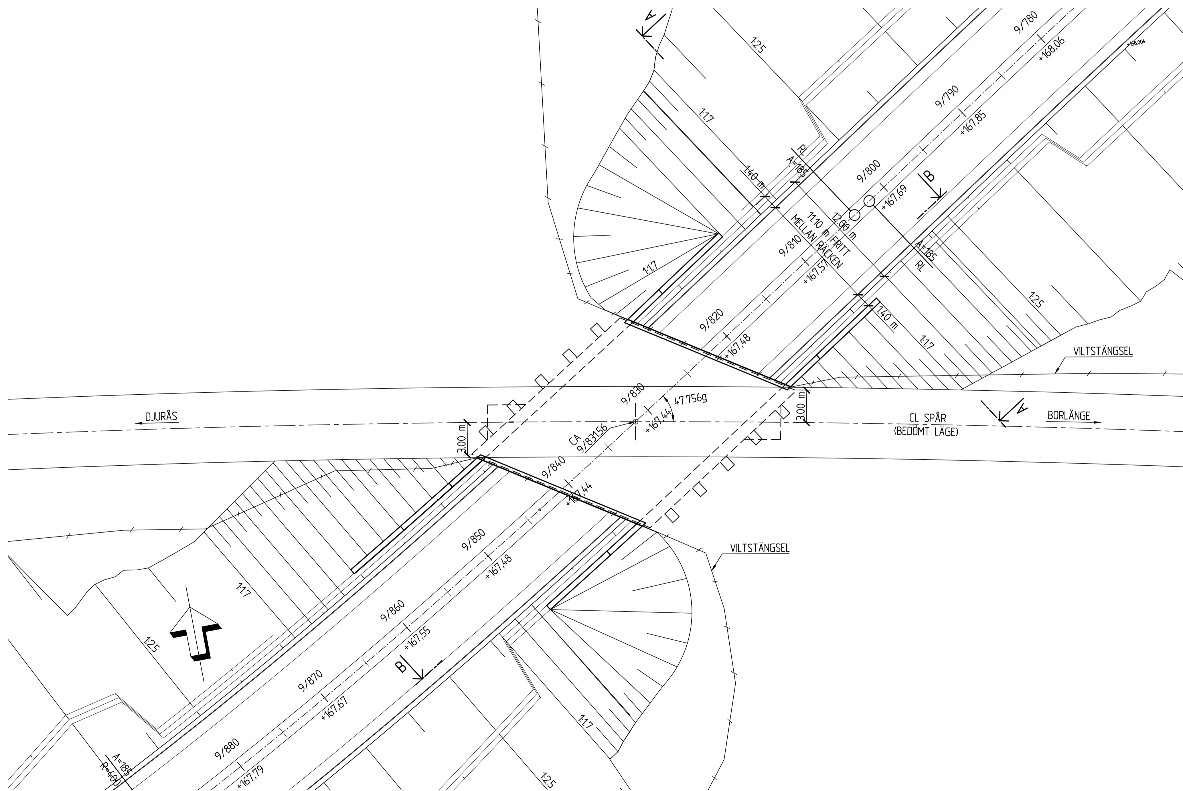
PLAN 1:200
