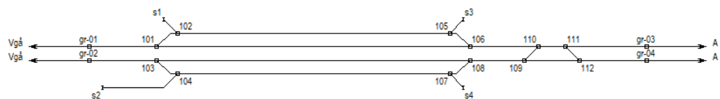
Figure 3 Track layout Algutsgården
