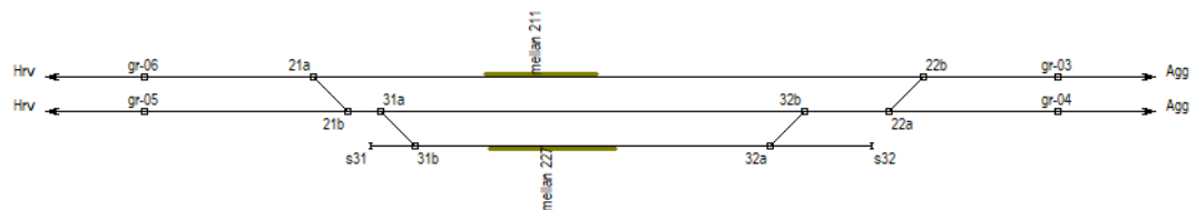
Figure 2 Track layout Vårgårda with platform locations
