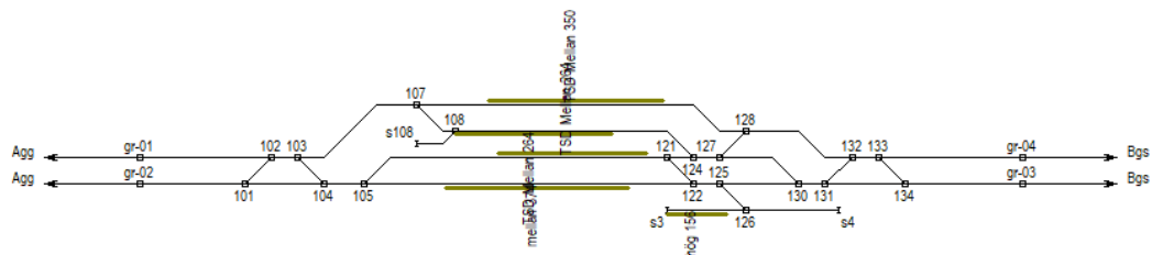
Figure 4 Track layout Alingsås with platform locations
