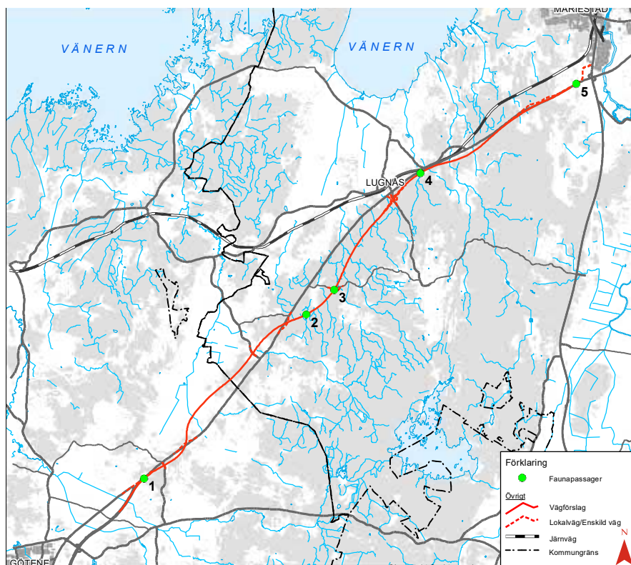
Figur 4.2.21. Planerade faunapassager.
