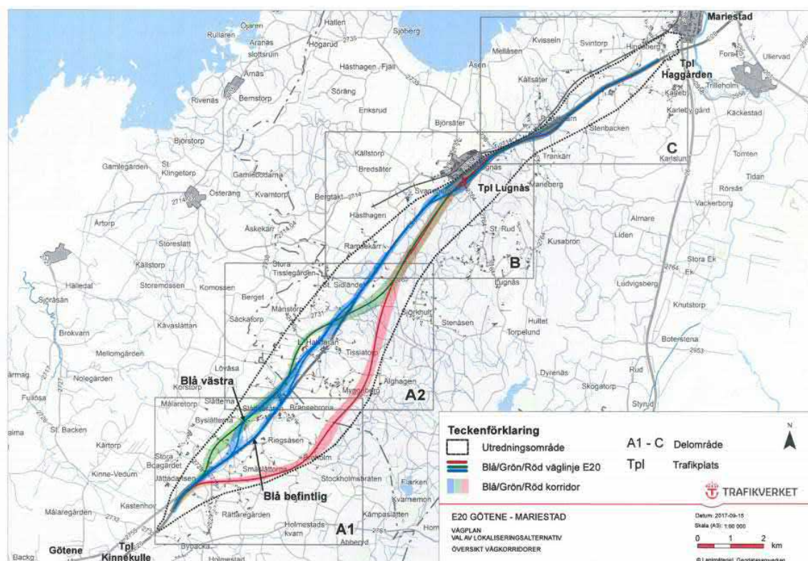
Figur 4.1.1 Korridorer E20 Götene–Mariestad.
