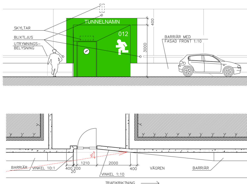
Figur 16 Plan utrymningsportal
